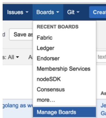
Fig. 30.1: Jira boards
